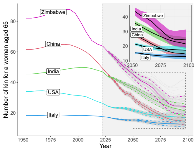
Fig. 2. Average number of living kin for a Focal woman aged 65 in selected countries. The gray lines in the background after 2021 show 100 trajectories from the 2022 Revision of the United Nations World Population Prospects. The continuous lines show the median of these projections, and the dashed lines indicate the 80% projection intervals.
