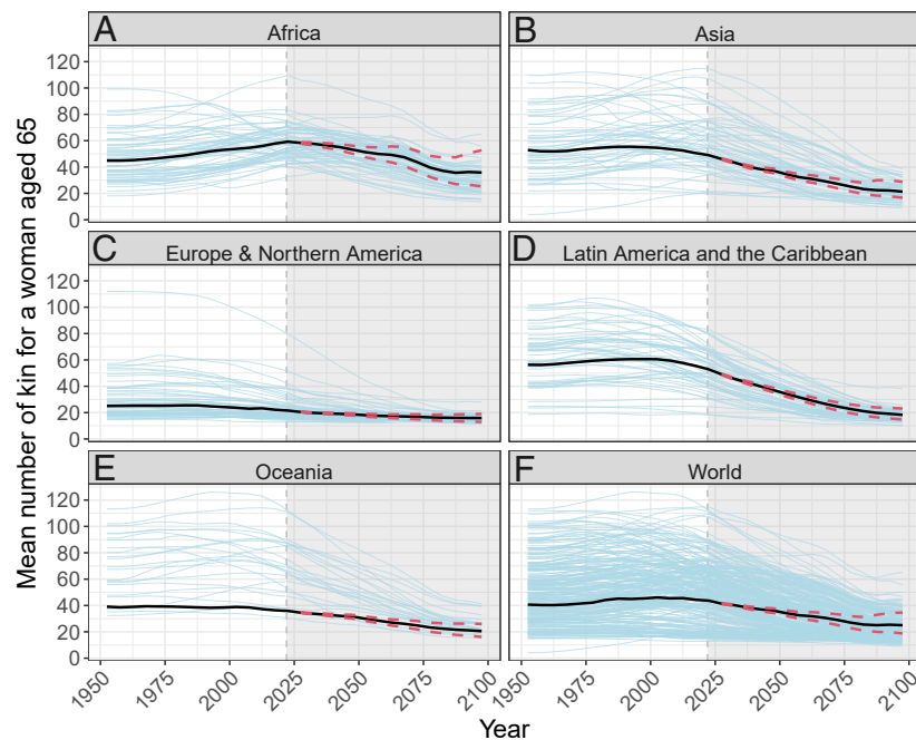
Fig. 1. Total family size the sum of all living great-grandparents, grandparents, parents, children, grandchildren, great-grandchildren, aunts/uncles, nieces/nephews (i.e., niblings), siblings, and cousins for a 65-yo female Focal in different world regions (Panels A–E) and globally (Panel F). The light-blue lines in the background show country-level values (median projection trajectory after 2021). The thick black lines indicate the regional values; after 2021, the black lines represent the projection median and the red lines represent the 80% projection intervals for each region (averages weighted by country-level population size at Focal's age 65).
