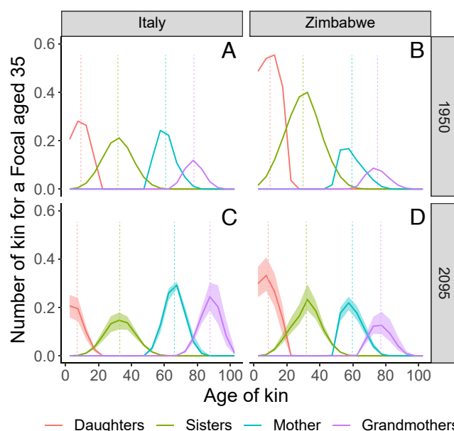
Fig. 4. Age composition of selected female relatives for a Focal woman aged 35 in Zimbabwe and Italy (1950 and 2095) ( A–D ). The shaded areas for 2095 show the 80% projection intervals of 1,000 individual probabilistic trajectories. The vertical lines indicate the mean age for each relative type.
