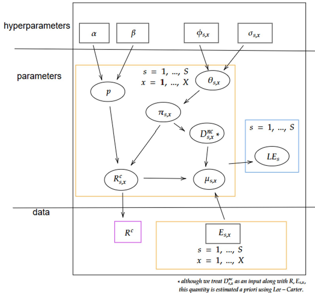
Fig. 1 A directed acyclic graph of the Bayesian model used to estimate life expectancy (LE). The ovals represent unknown parameters and the rectangles represent the available data used as inputs. The colors of the boxes represent the different dimensions of the parameters and data, with purple denoting a scalar value, orange denoting multidimensional arrays (age-sex), and blue denoting a one dimensional array (sex). The hyperparameters for the reporting rate and the age distributions are specified based on information elicited from prior and current work. We note that D^{nc}_{s,x} before Oct. 7th, 2023 is not included in the DAG; however, it may impact the estimation of \pi_{s,x} (i.e. when estimating \pi_{s,x} from B'tselem's historical average)
